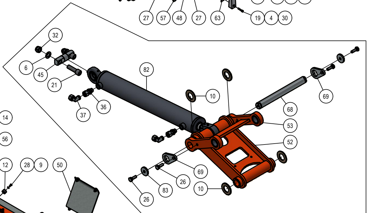
Detail opklapcilinder
