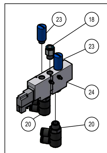
Detail A
